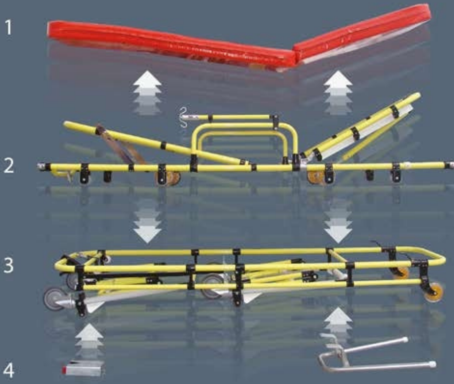
Transferli Ana Sedye bileşenleri Transfer Main Stretcher components
